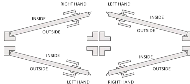
Handing for Emergency Escape Lock
