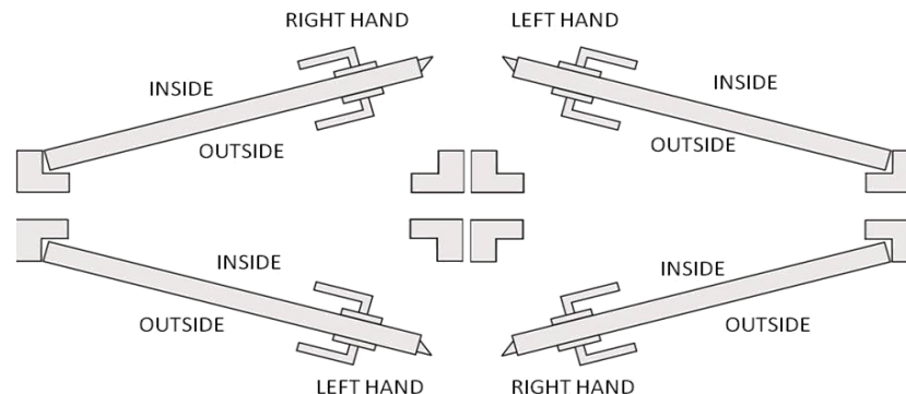
Handing for Emergency Escape Lock
